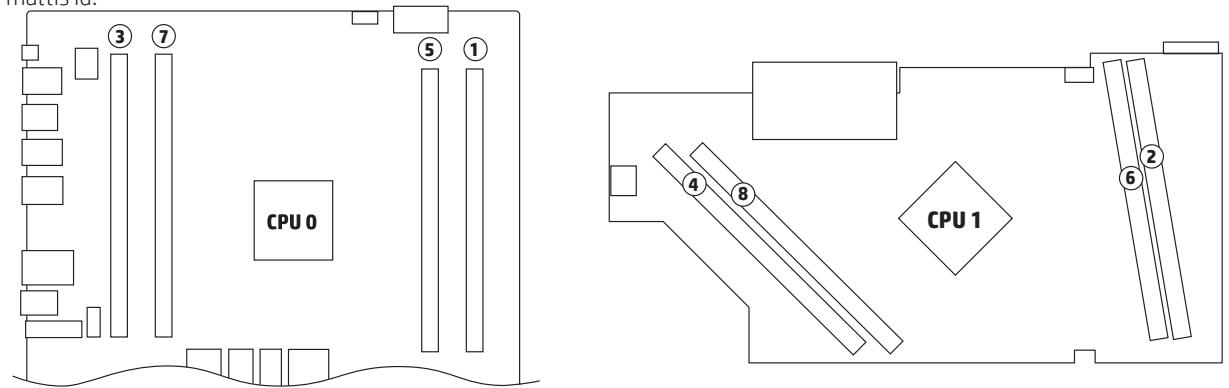
Figure 6. Loading order for dual CPU configurations
